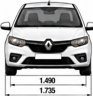
VISTA FRONTAL
